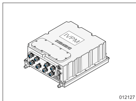
Figure 2: “SIEMENS” voltage inverter with built-in overvoltage protection
