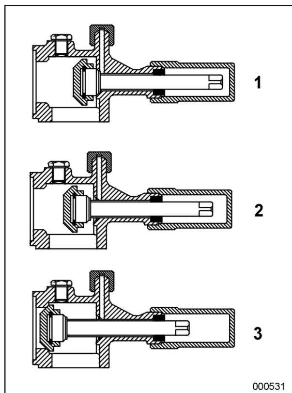
Figure 3: Service valve positions
